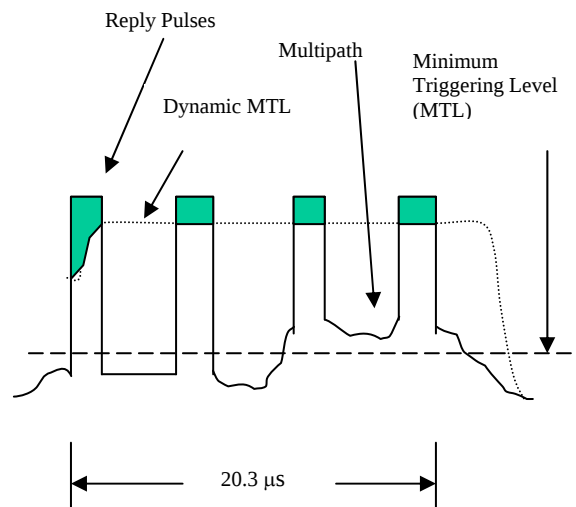
Figure 8. Dynamic Thresholding of ATCRBS Replies
