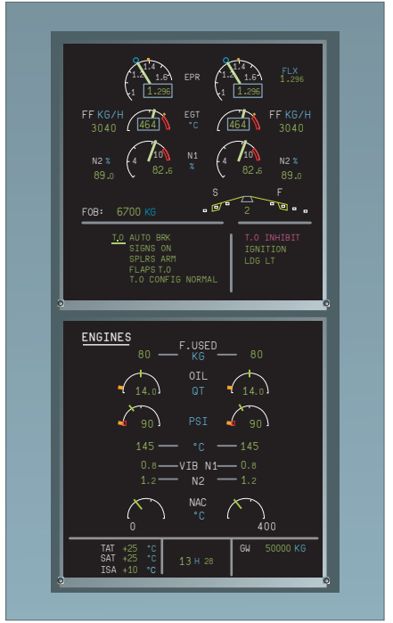
IAE engines
